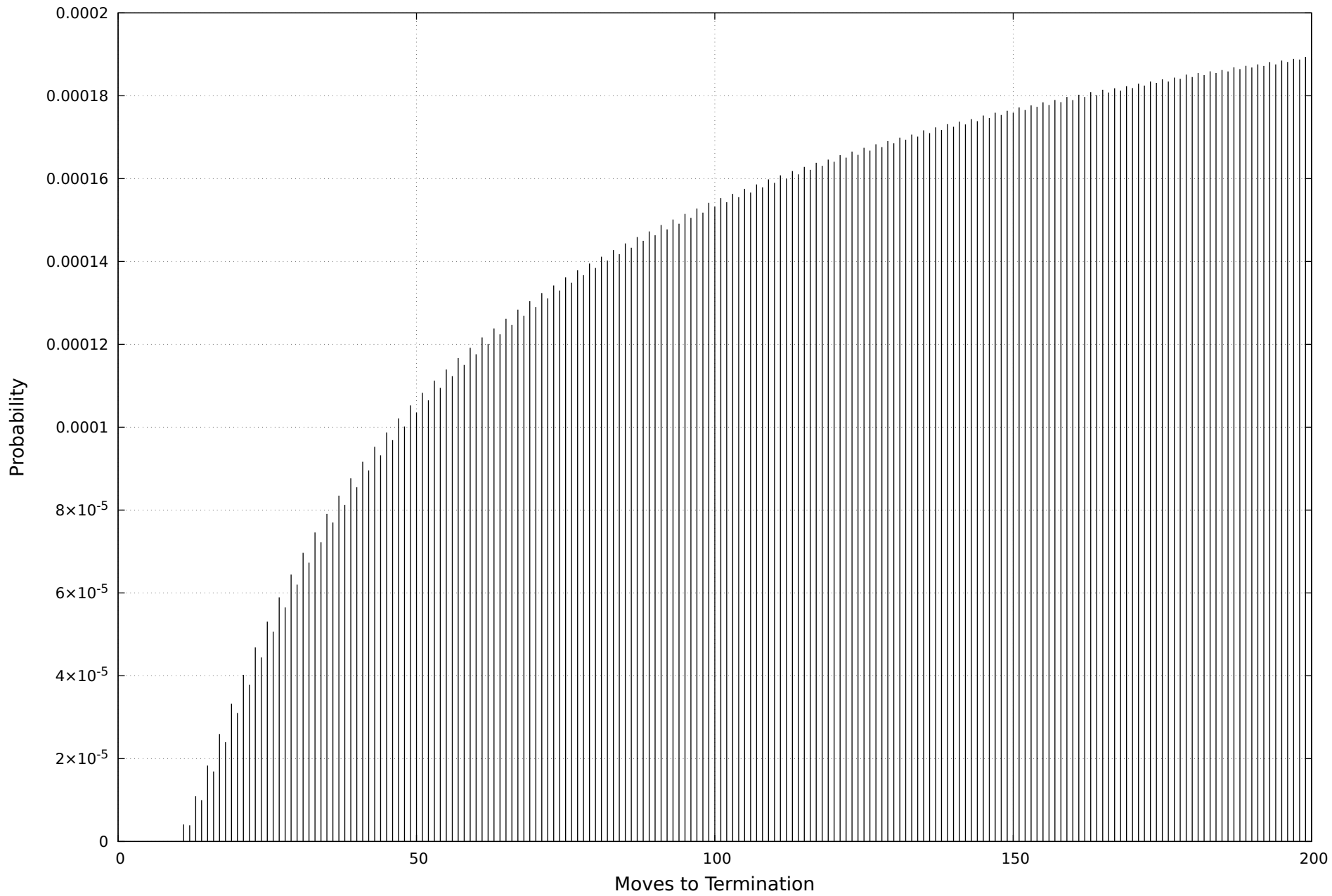
Self-Trapping Random Walk on 3-D Lattice ( 27 \cdot 10^9 Walks)
