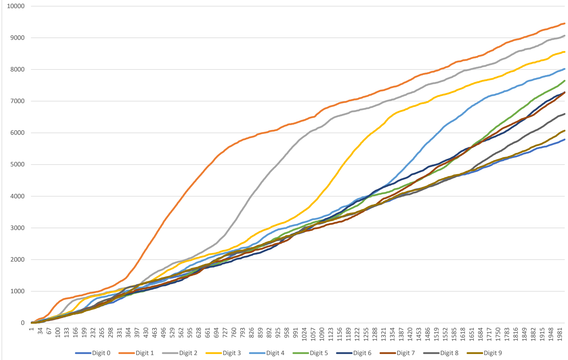
Digit charts for the first 20000 terms
