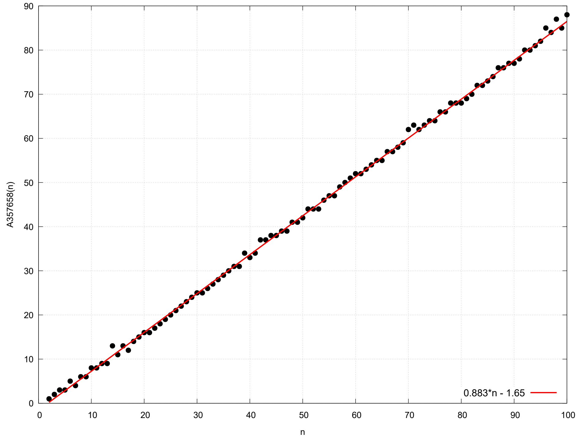
Maximum number of bits=1 in squares 2^n < k^2 < 2^{n+1}
