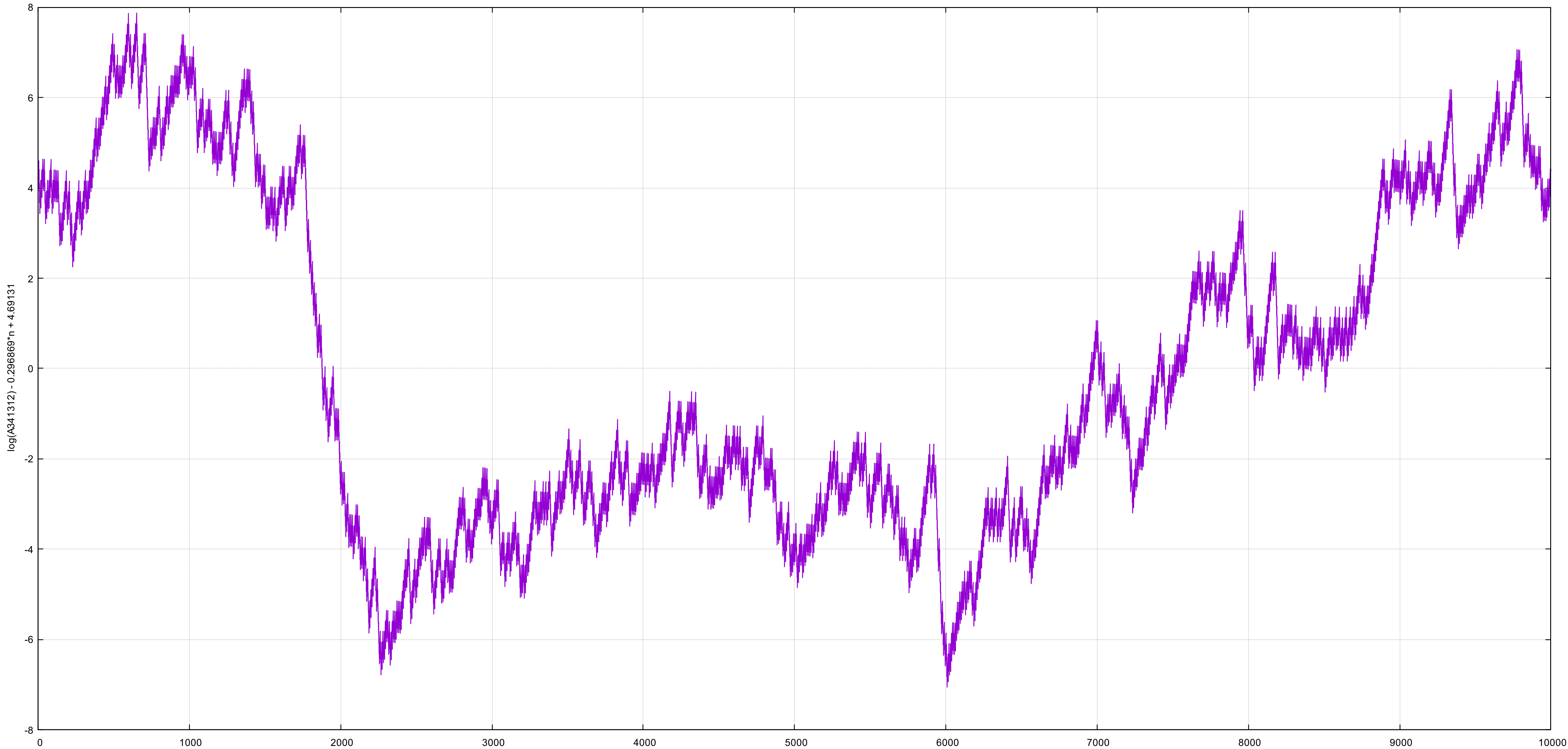
Deviation of \log(A_{341312}) from linear fit in range 3...10000
