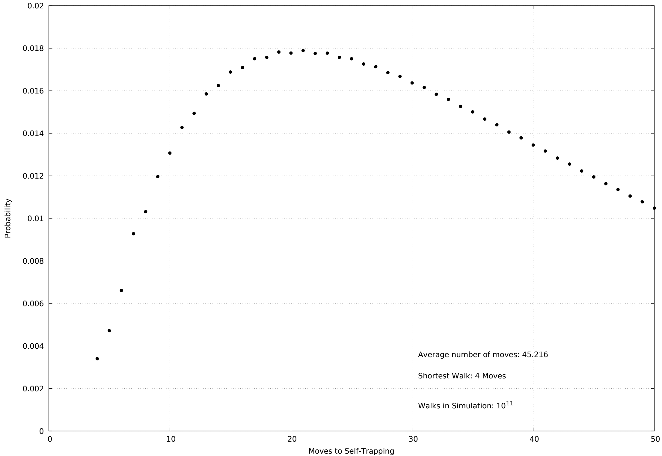
Self-Avoiding Uncrossed Knight's Walks
