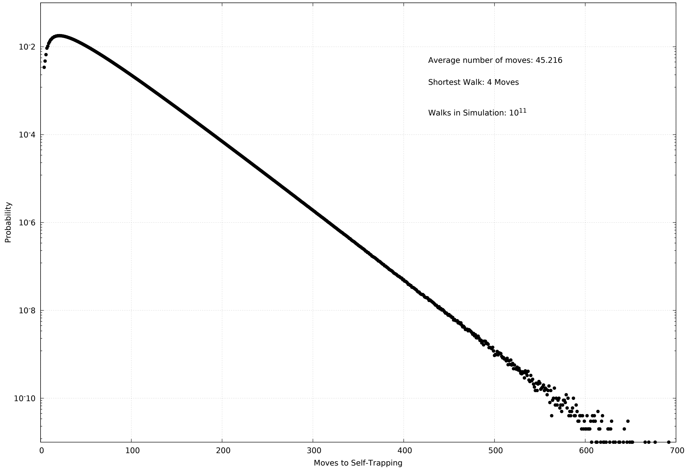
Self-Avoiding Uncrossed Knight's Walks
