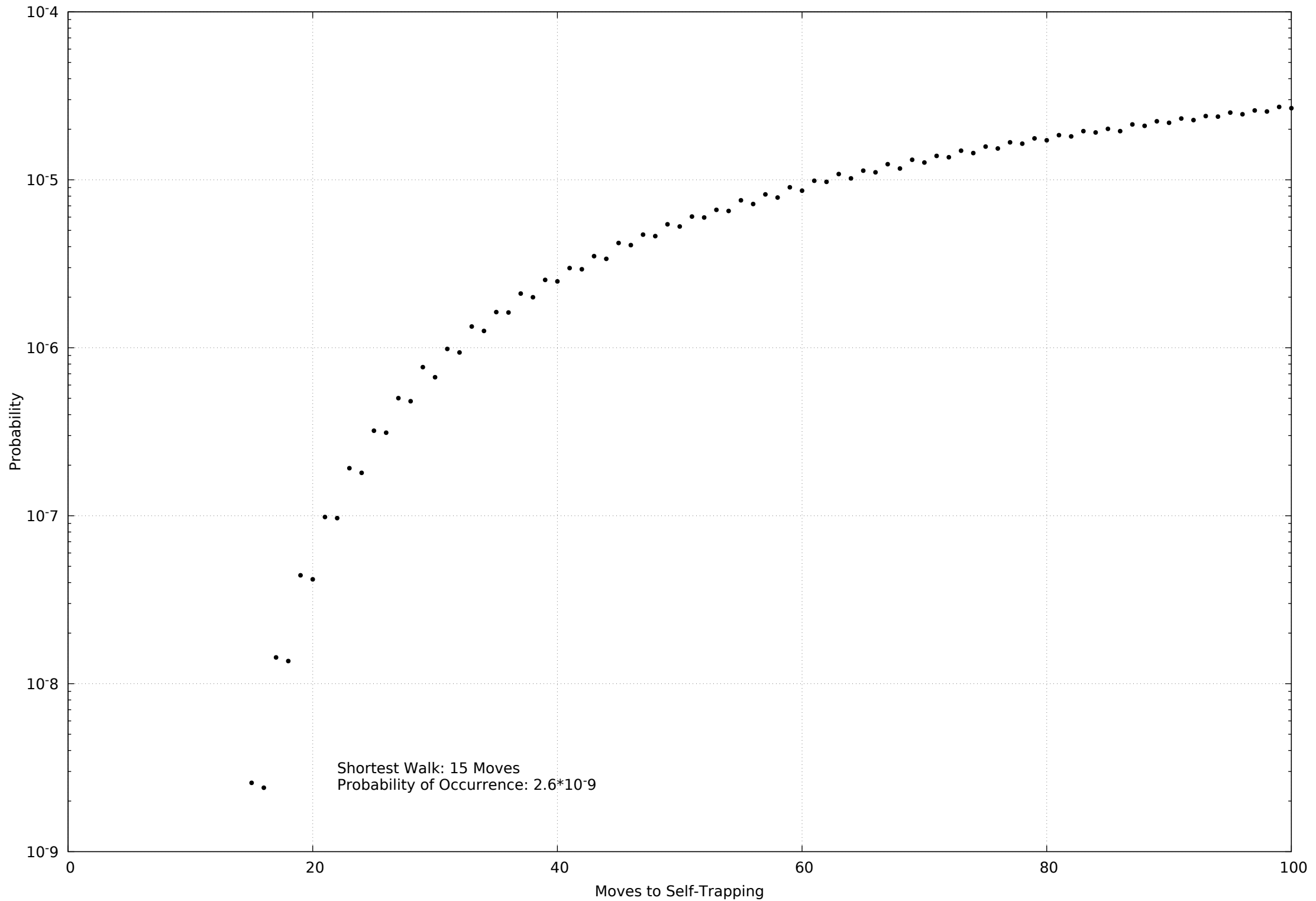
Self-Avoiding Knight's Walks
