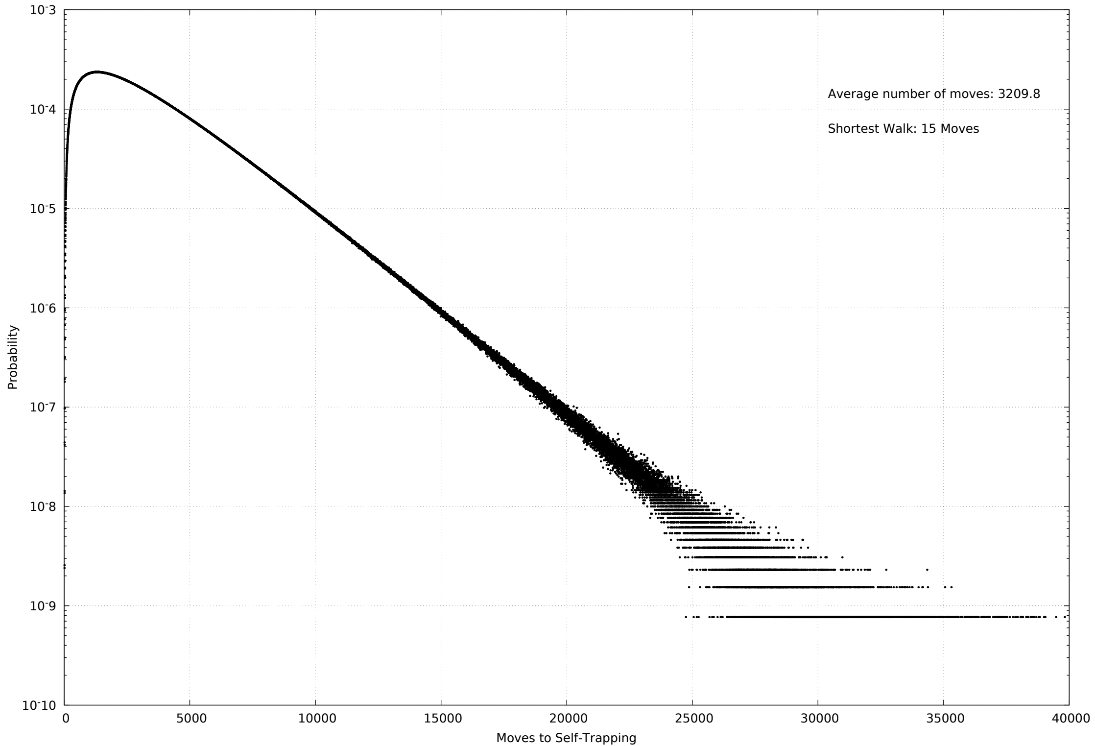
Self-Avoiding Knight's Walks
