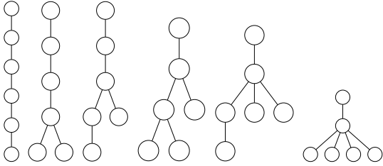
6 trees on 6 nodes
