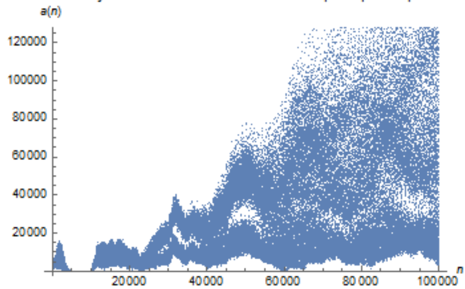
Number of ways to write n as an ordered sum of 5 prime power palindromes
