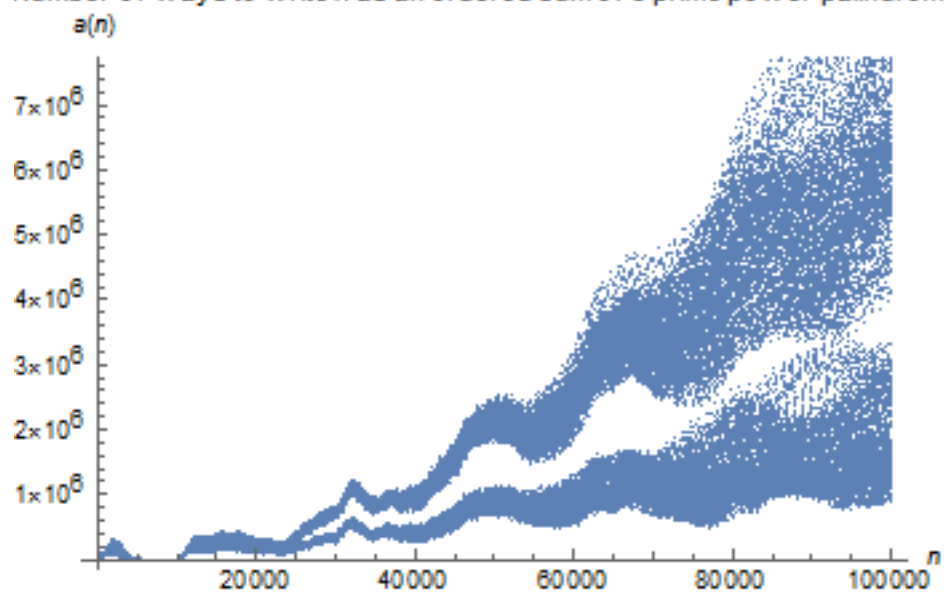
Number of ways to write n as an ordered sum of 6 prime power palindromes
