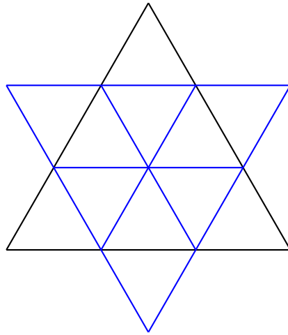
Figure 1: Level 1 and 2 approximations to Koch fractal triangulation (interior included), ratio = \frac{1}{3}
