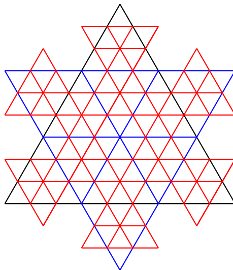
Figure 2: Level 1, 2 and 3 approximations to von Koch fractal triangulation, ratio = \frac{1}{3}
