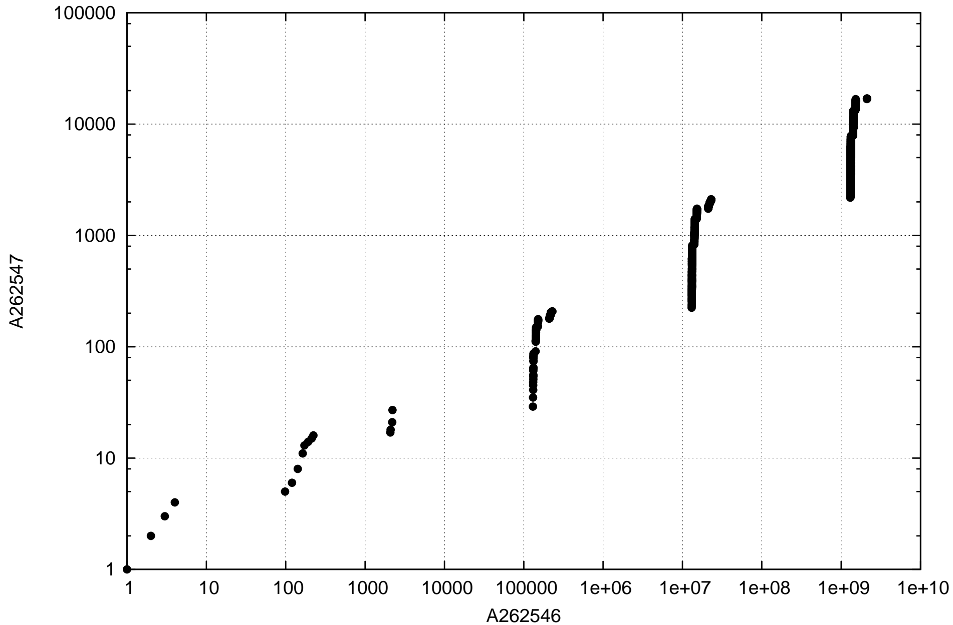
Least number of representations by sums of 3 palindromes
