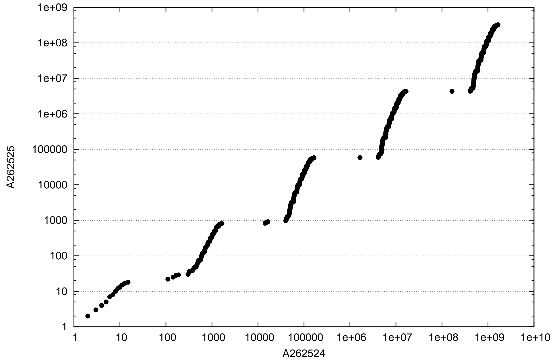
Records in the number of representations by the sum of 3 palindromes
