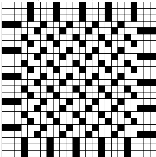
Figure 22: n = 24 , 268 clues
