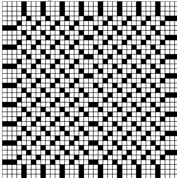
Figure 35: n = 37 , 642 clues
