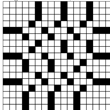
Figure 15: n = 17 , 126 clues
