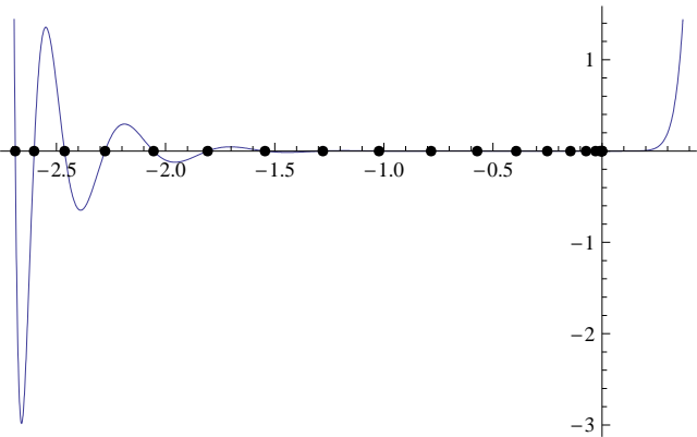
The 20 negative real roots of P(20,x)
