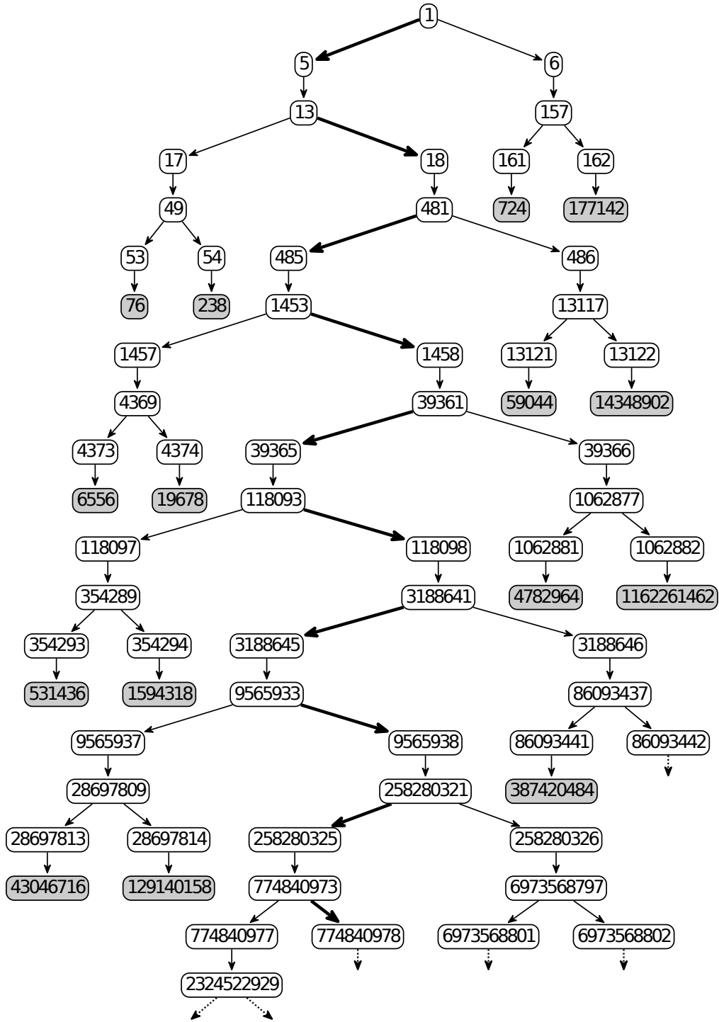
FIGURE 4. A portion of the base-3 child graph G_c . The thick lines are the start of the unique infinite path (A367621). The shaded nodes are the landmines, which must be avoided. Short vertical arrows represent long unbranched paths.
