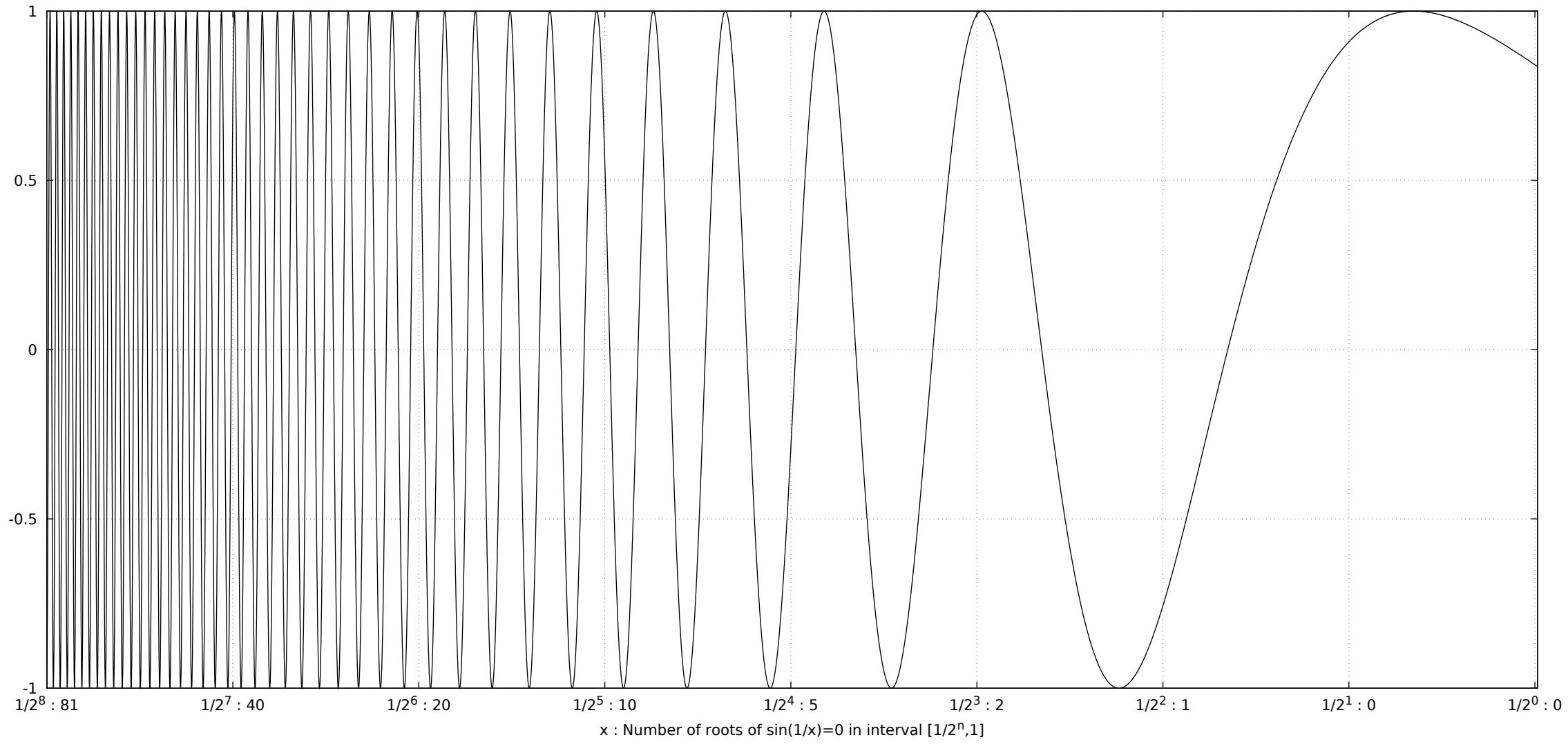
sin (1/x) plotted on logarithmic x-axis
