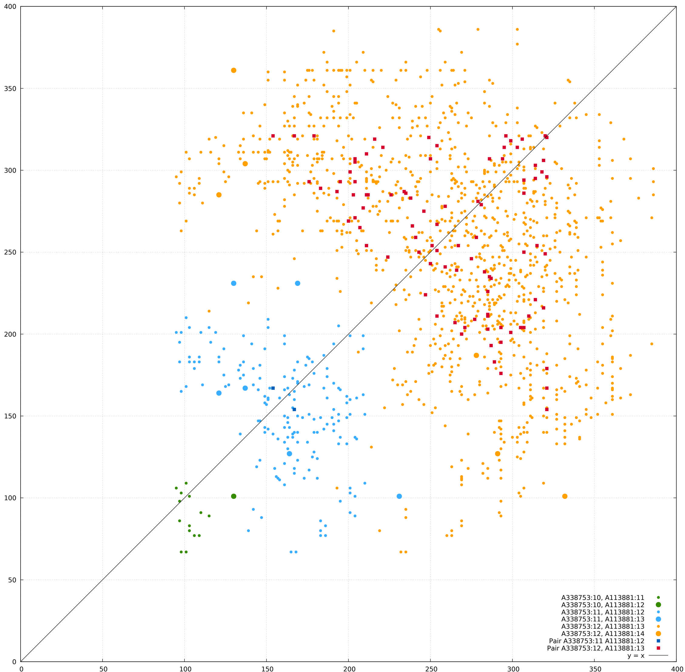
Where A338753 differs from A113881, x, y \leq 380
