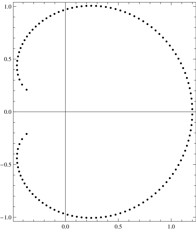
Roots of p(120,x)
